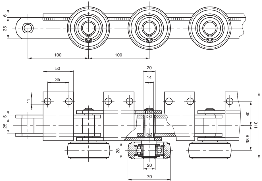
Chain P. 100x25x22 øB
